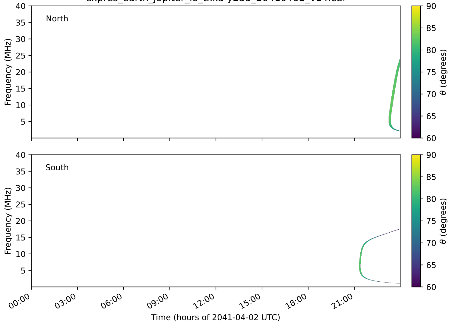
expres_earth_jupiter_io_txka-y235_20410402_v14.cdf
