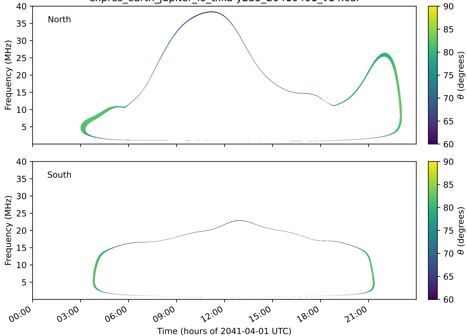
expres_earth_jupiter_io_txka-y235_20410401_v14.cdf
