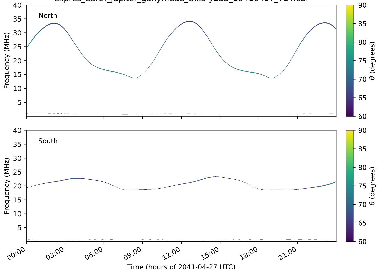
expres_earth_jupiter_ganymede_txka-y235_20410427_v14.cdf
