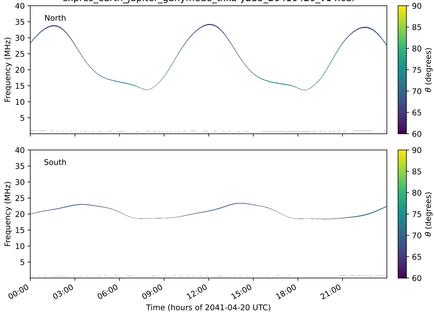
expres_earth_jupiter_ganymede_txka-y235_20410420_v14.cdf
