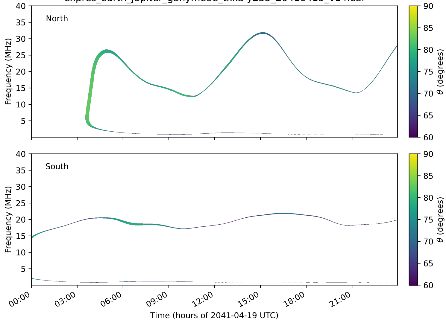
expres_earth_jupiter_ganymede_txka-y235_20410419_v14.cdf
