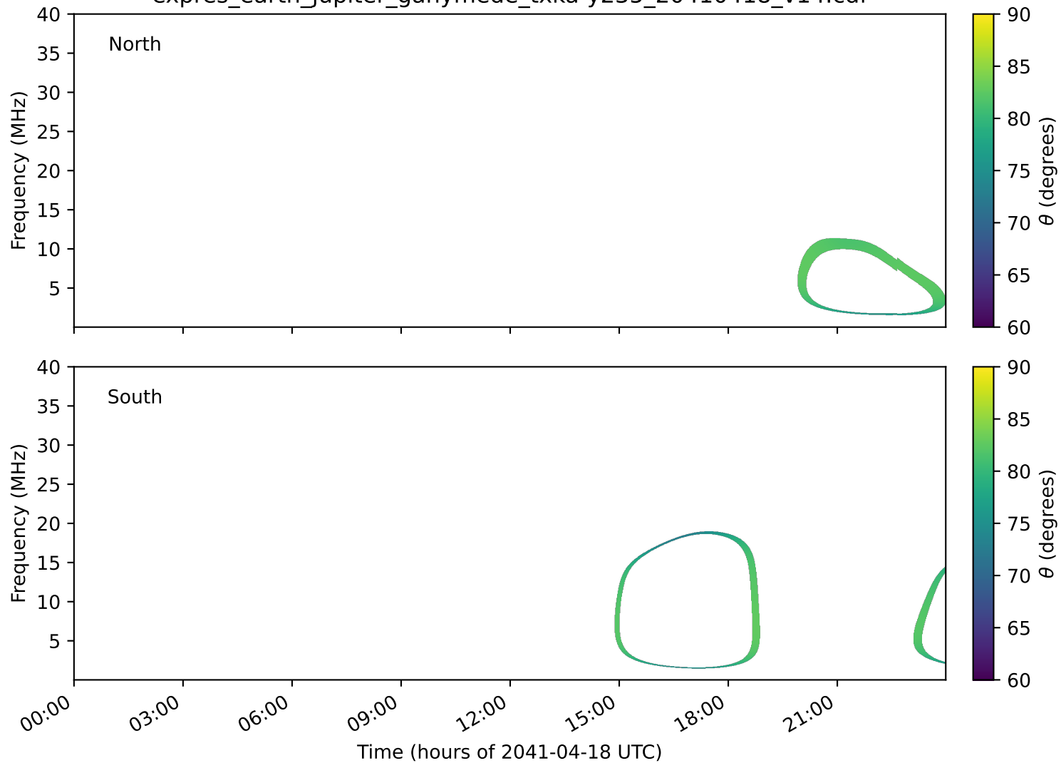
expres_earth_jupiter_ganymede_txka-y235_20410418_v14.cdf
