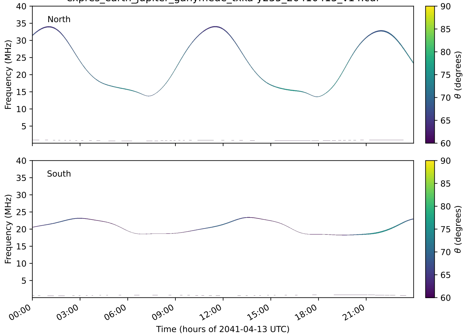
expres_earth_jupiter_ganymede_txka-y235_20410413_v14.cdf
