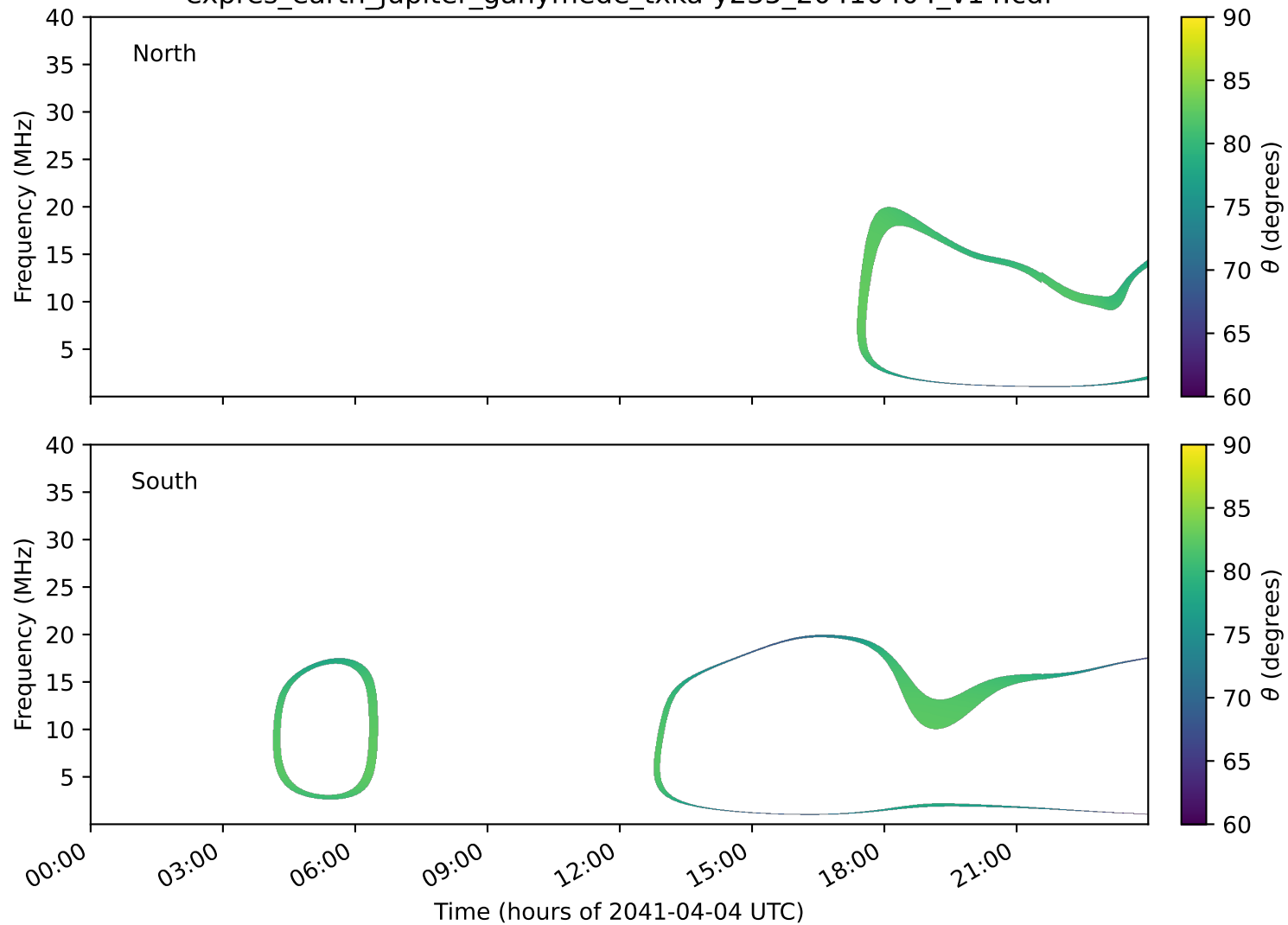
expres_earth_jupiter_ganymede_txka-y235_20410404_v14.cdf
