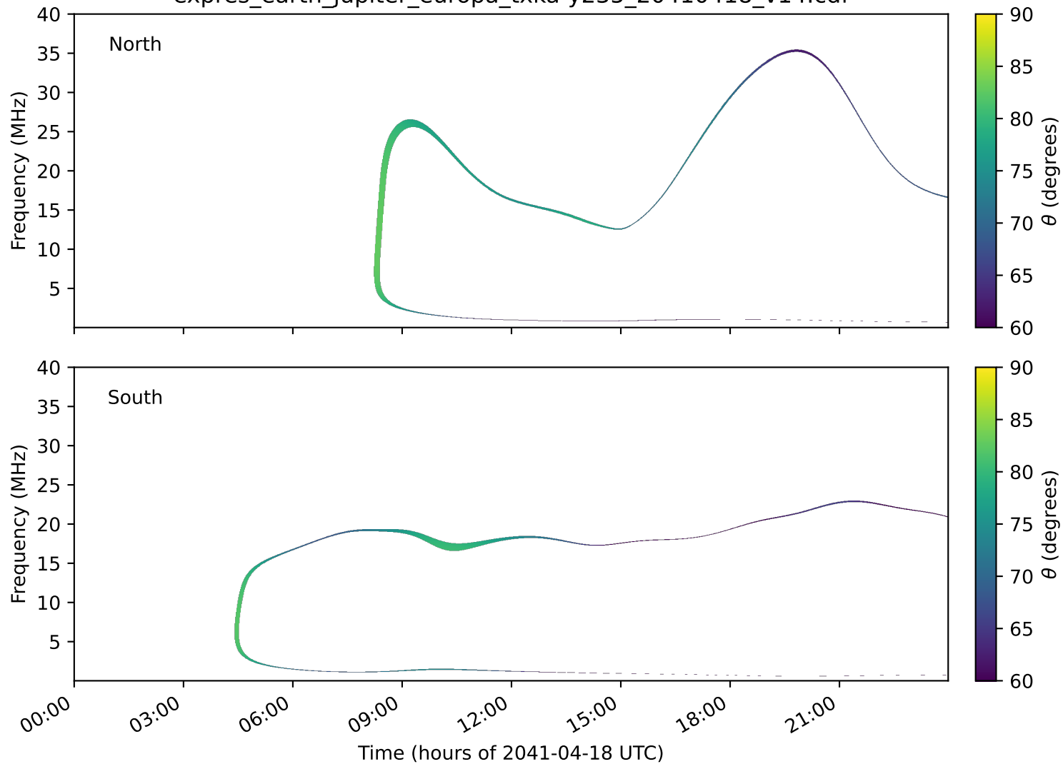
expres_earth_jupiter_europa_txka-y235_20410418_v14.cdf
