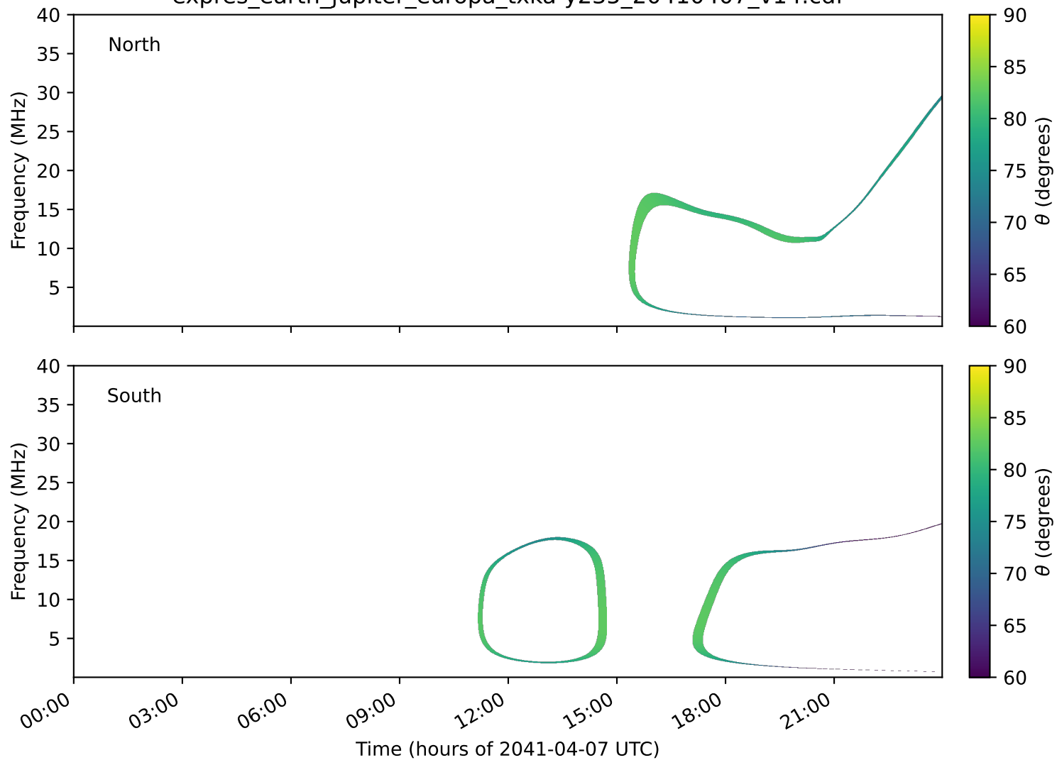
expres_earth_jupiter_europa_txka-y235_20410407_v14.cdf
