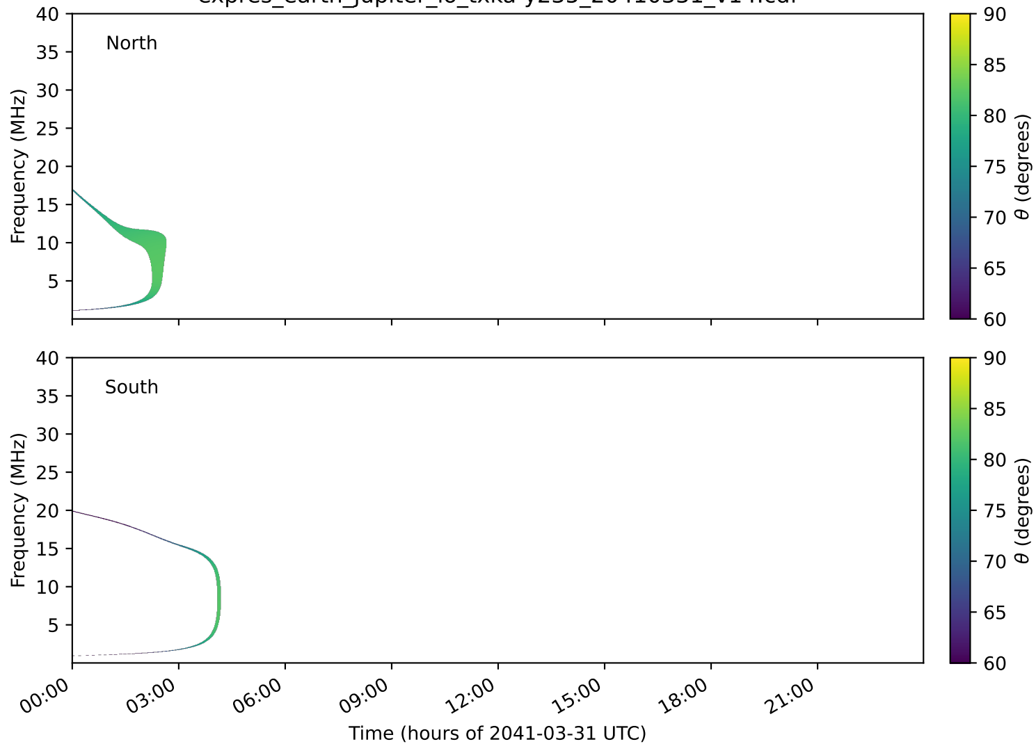
expres_earth_jupiter_io_txka-y235_20410331_v14.cdf
