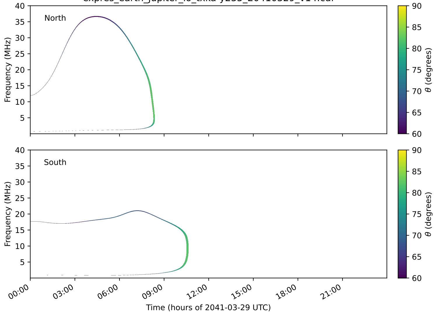
expres_earth_jupiter_io_txka-y235_20410329_v14.cdf
