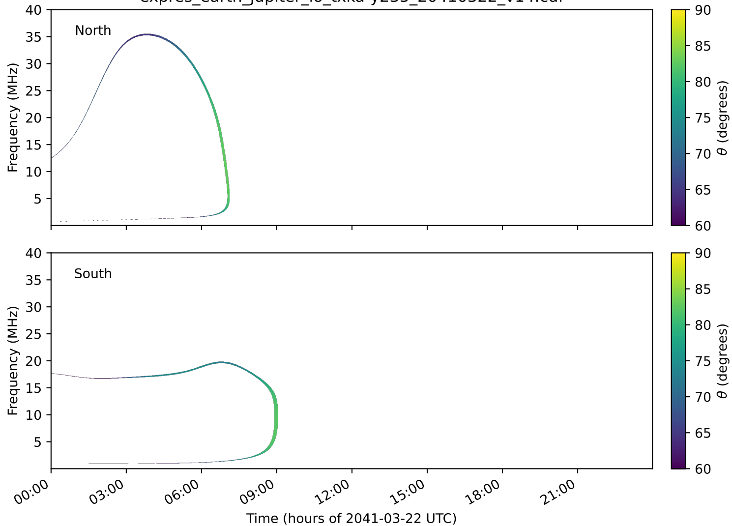
expres_earth_jupiter_io_txka-y235_20410322_v14.cdf
