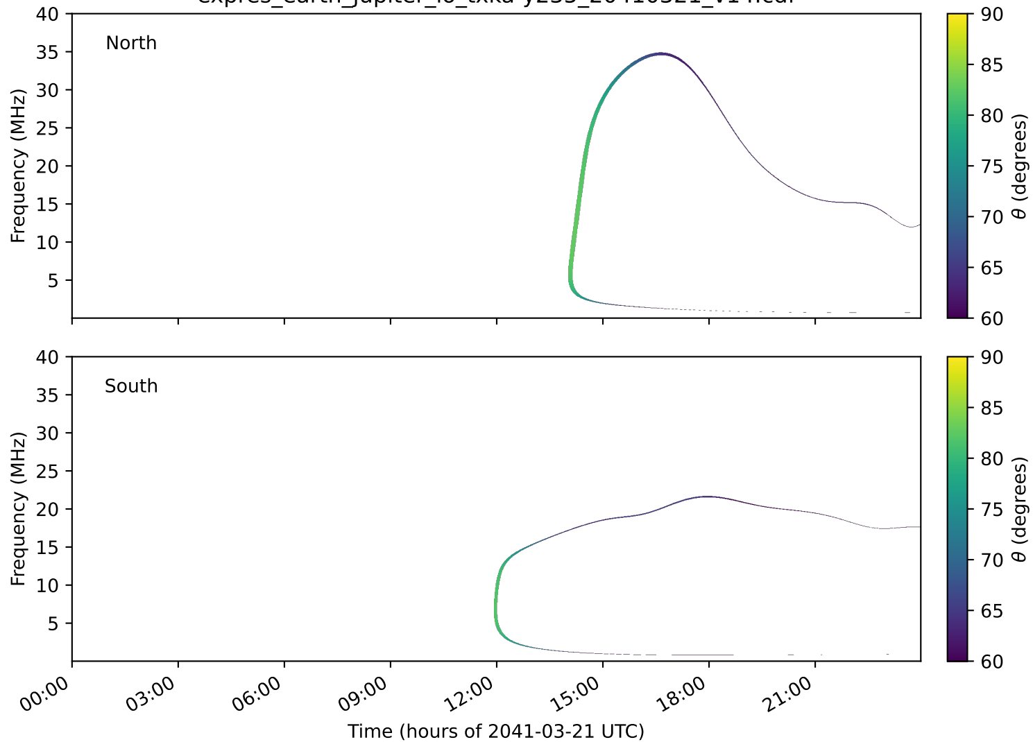
expres_earth_jupiter_io_txka-y235_20410321_v14.cdf
