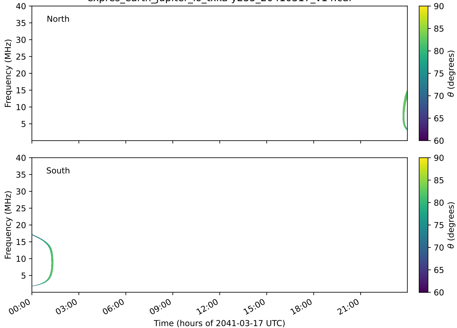
expres_earth_jupiter_io_txka-y235_20410317_v14.cdf
