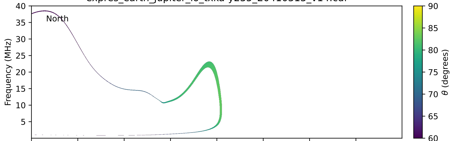
expres_earth_jupiter_io_txka-y235_20410313_v14.cdf
