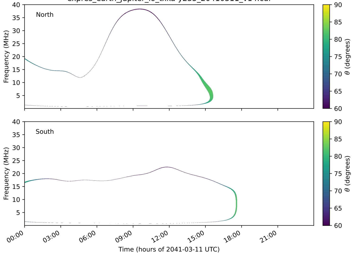
expres_earth_jupiter_io_txka-y235_20410311_v14.cdf
