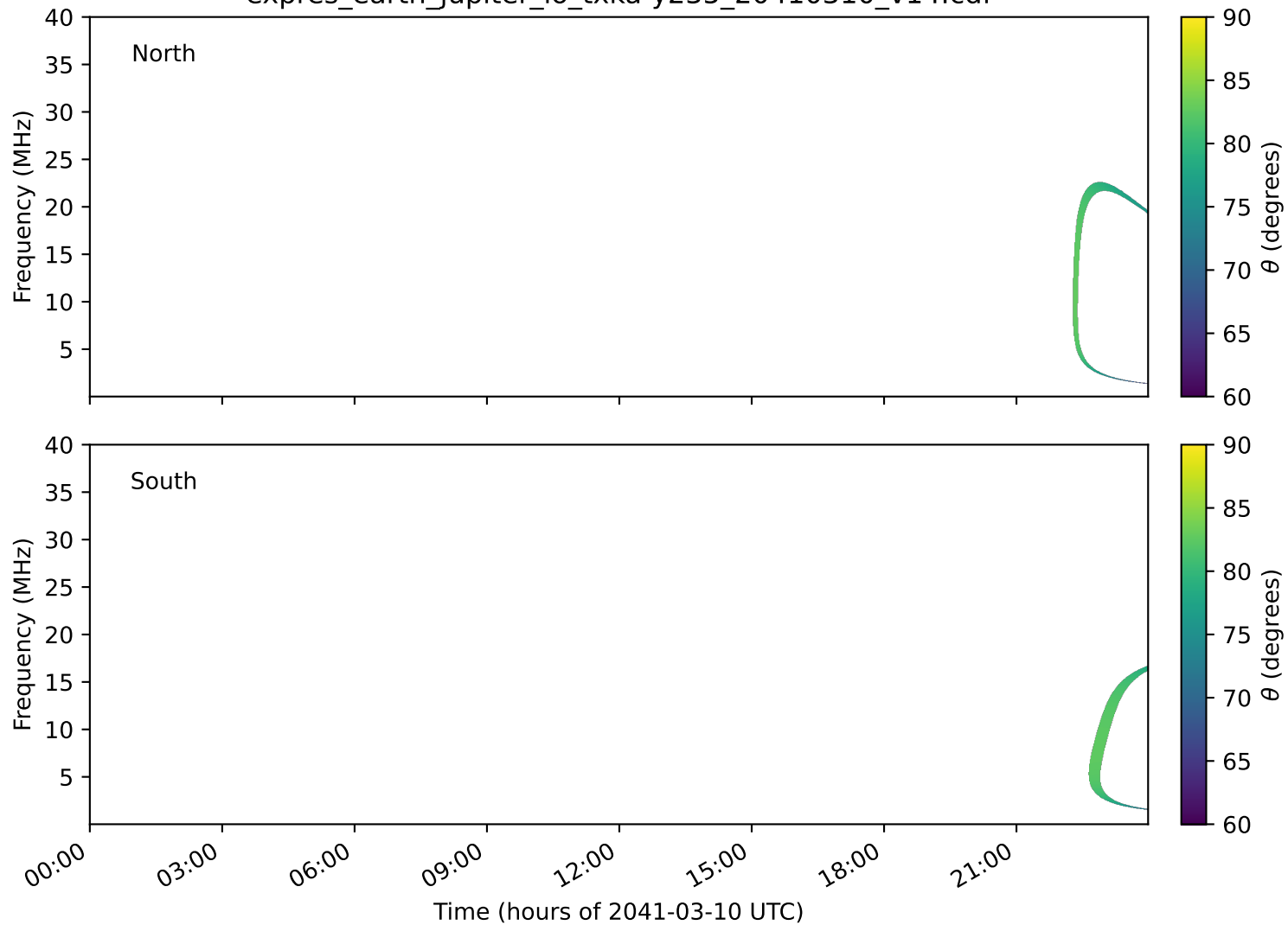
expres_earth_jupiter_io_txka-y235_20410310_v14.cdf
