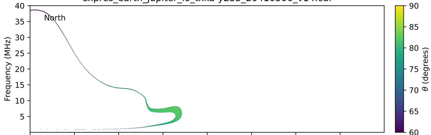
expres_earth_jupiter_io_txka-y235_20410306_v14.cdf
