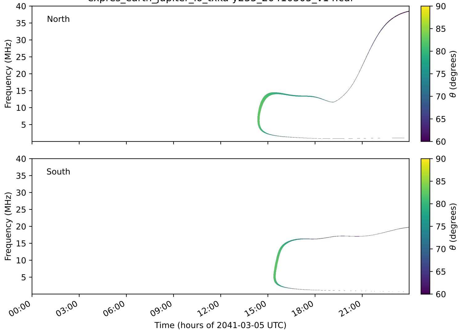
expres_earth_jupiter_io_txka-y235_20410305_v14.cdf
