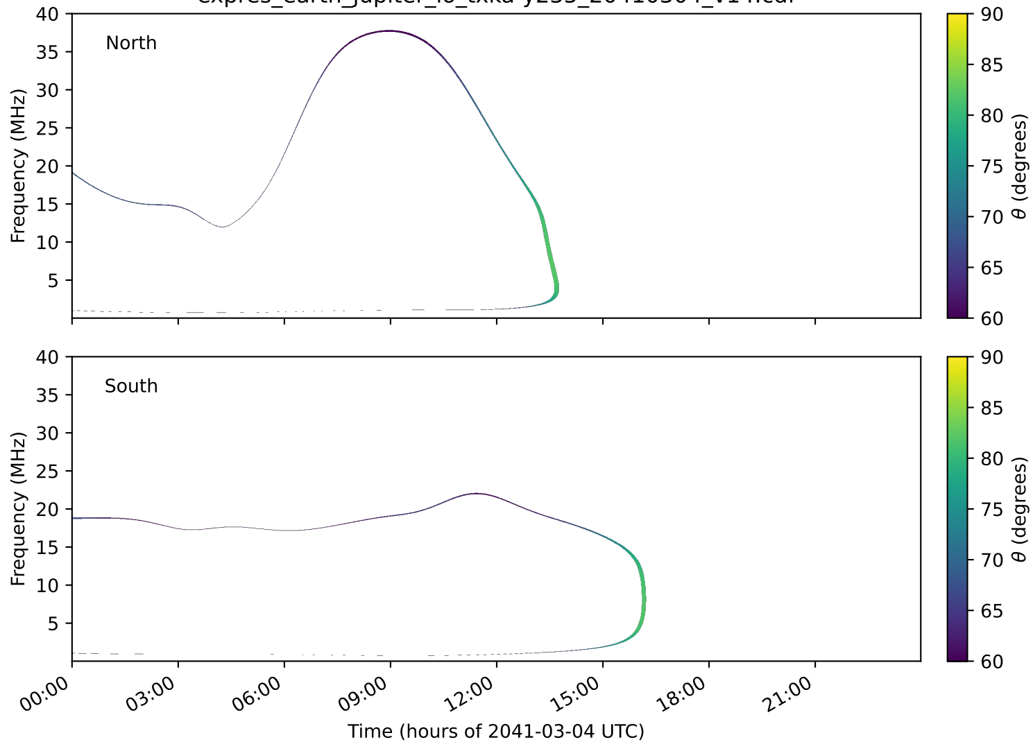
expres_earth_jupiter_io_txka-y235_20410304_v14.cdf
