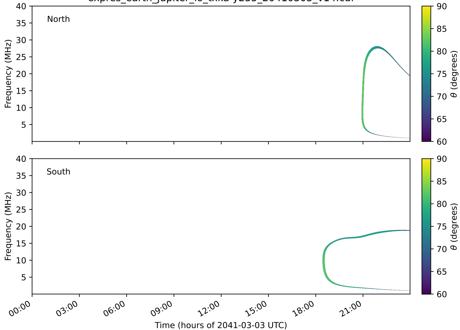
expres_earth_jupiter_io_txka-y235_20410303_v14.cdf
