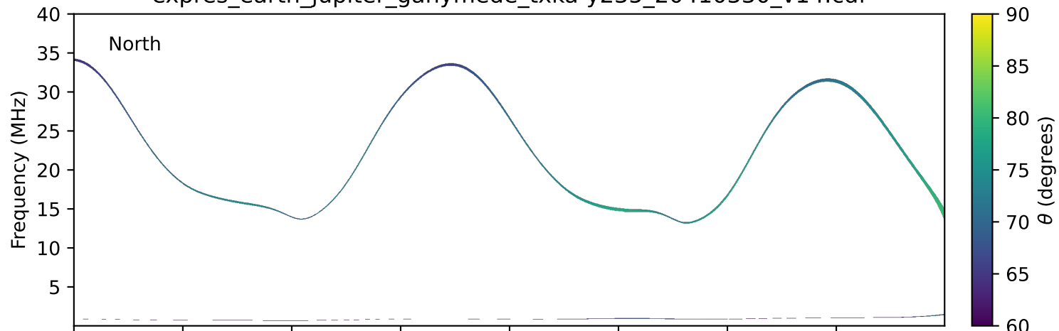
expres_earth_jupiter_ganymede_txka-y235_20410330_v14.cdf
