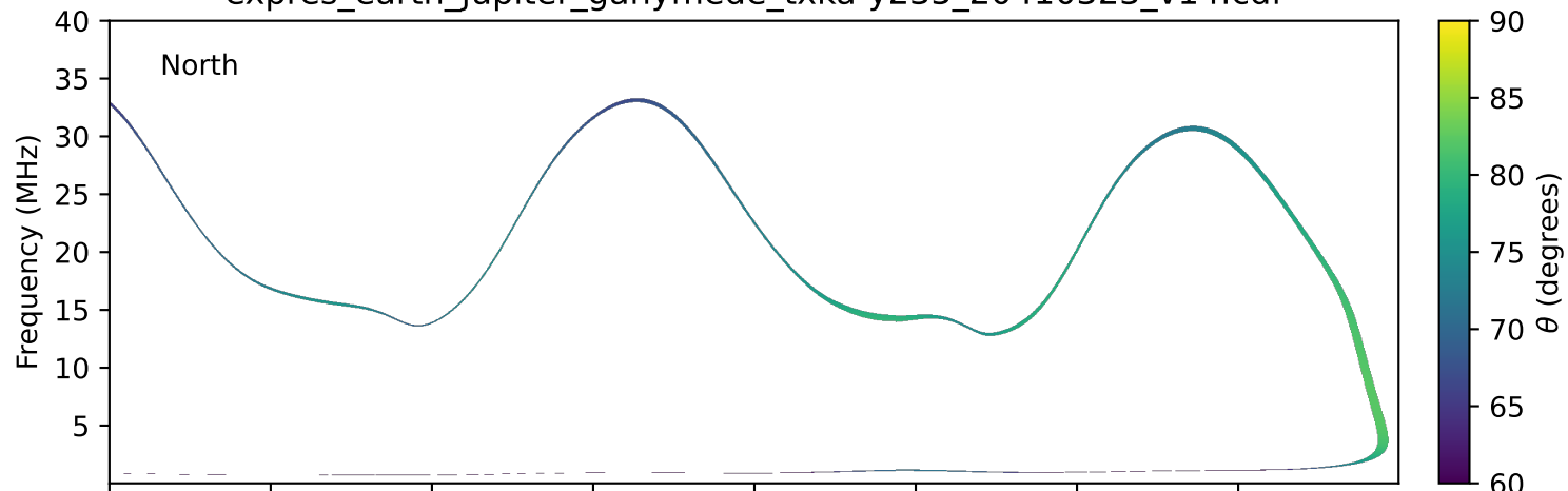
expres_earth_jupiter_ganymede_txka-y235_20410323_v14.cdf
