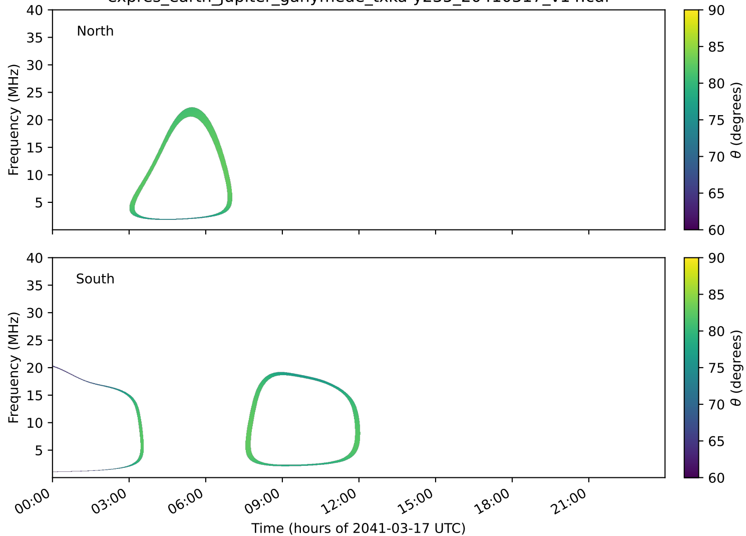
expres_earth_jupiter_ganymede_txka-y235_20410317_v14.cdf
