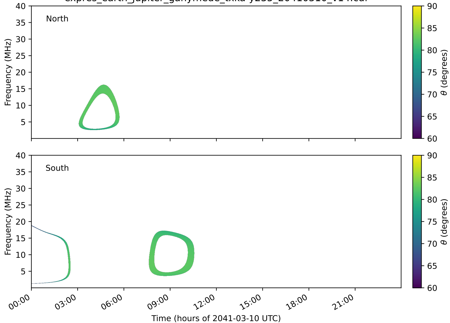
expres_earth_jupiter_ganymede_txka-y235_20410310_v14.cdf
