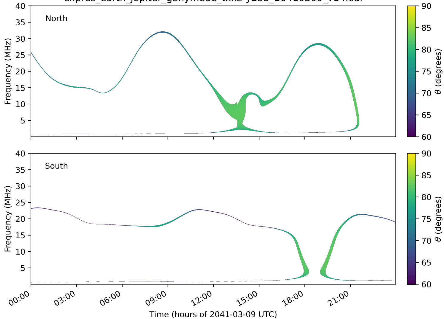
expres_earth_jupiter_ganymede_txka-y235_20410309_v14.cdf
