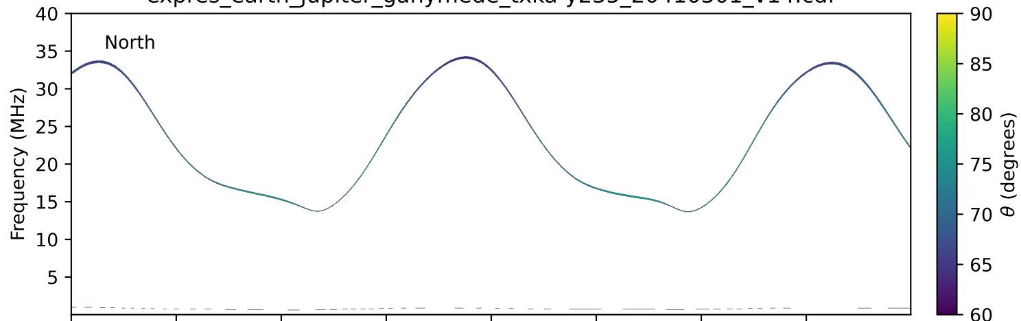
expres_earth_jupiter_ganymede_txka-y235_20410301_v14.cdf
