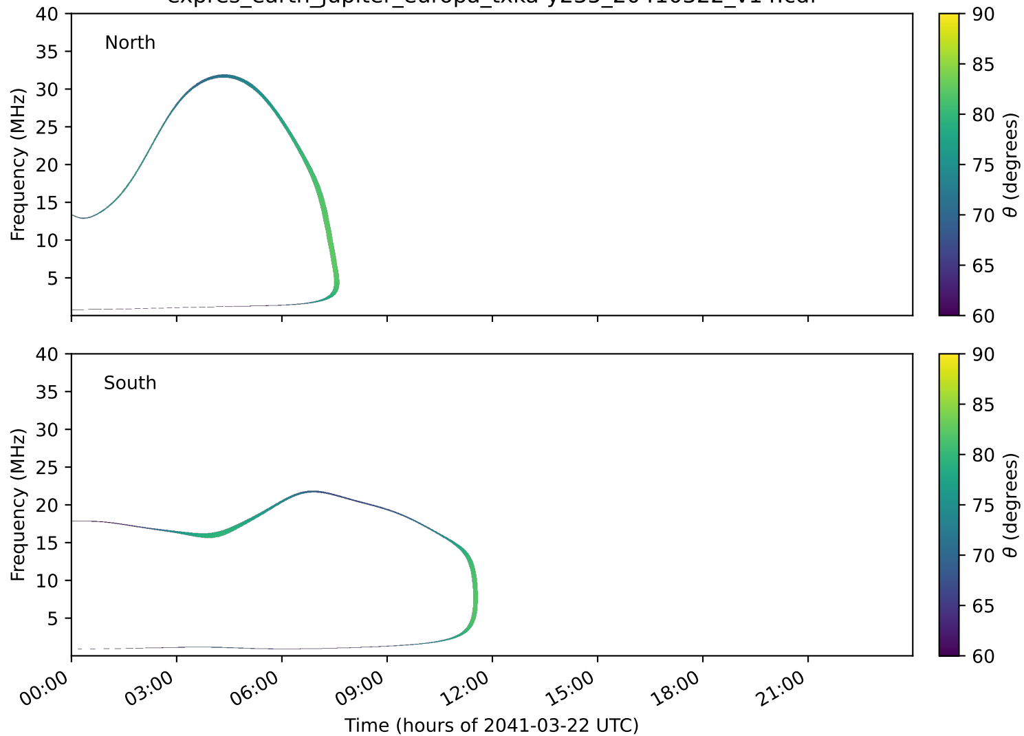
expres_earth_jupiter_europa_txka-y235_20410322_v14.cdf
