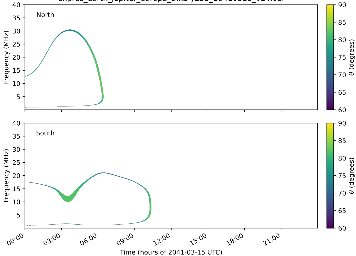
expres_earth_jupiter_europa_txka-y235_20410315_v14.cdf
