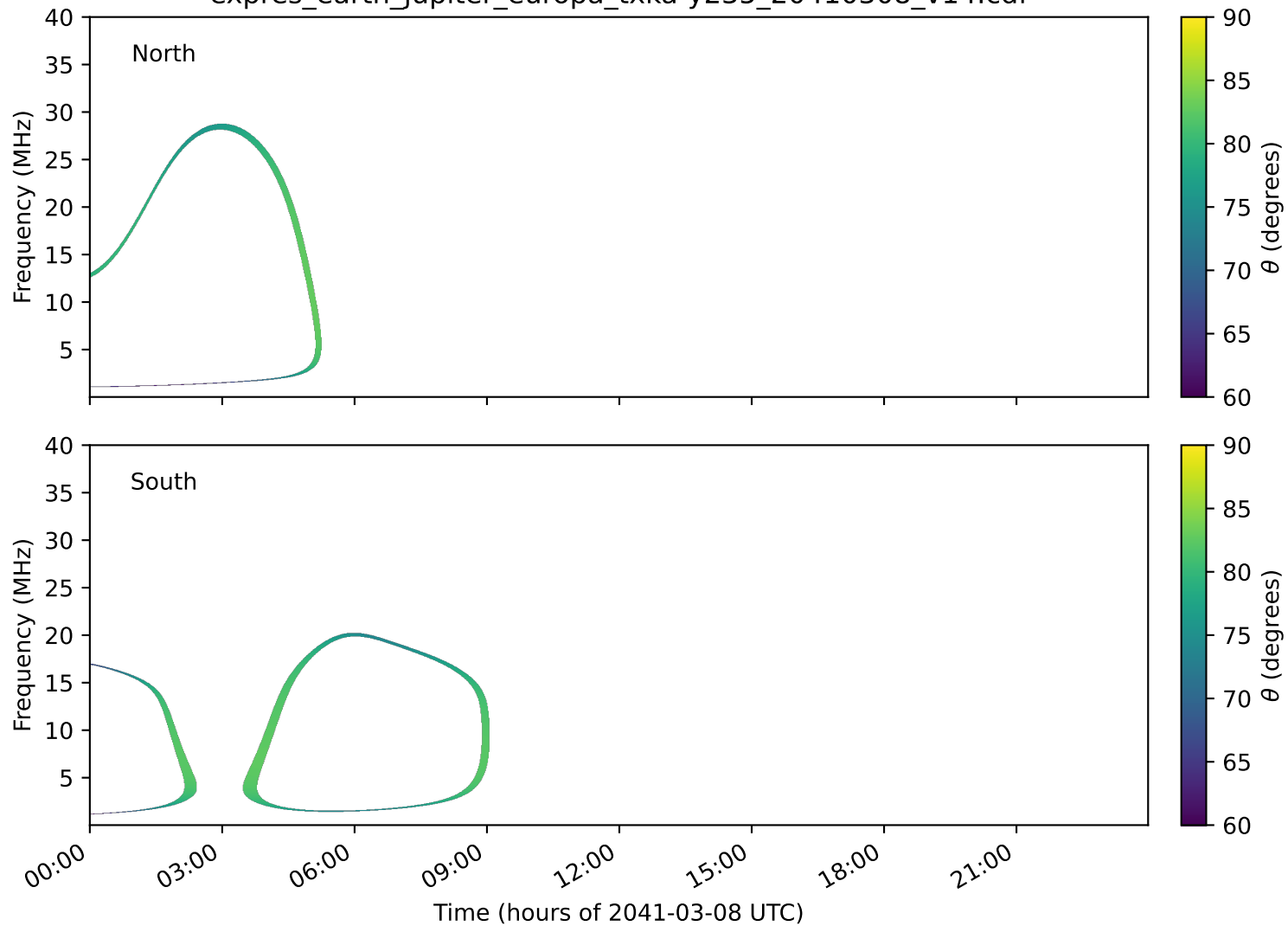
expres_earth_jupiter_europa_txka-y235_20410308_v14.cdf
