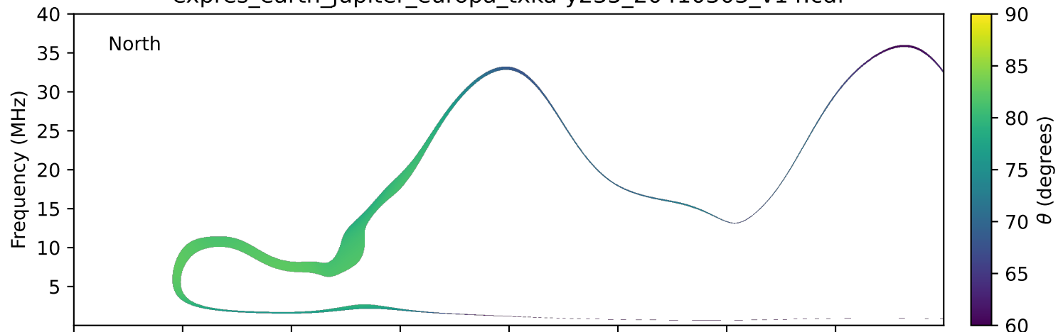
expres_earth_jupiter_europa_txka-y235_20410303_v14.cdf
