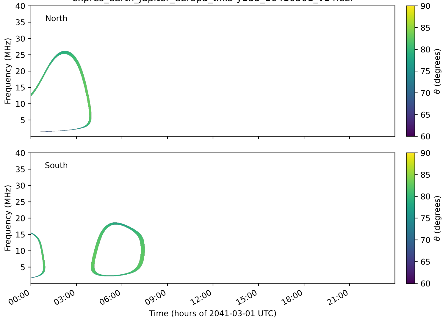
expres_earth_jupiter_europa_txka-y235_20410301_v14.cdf
