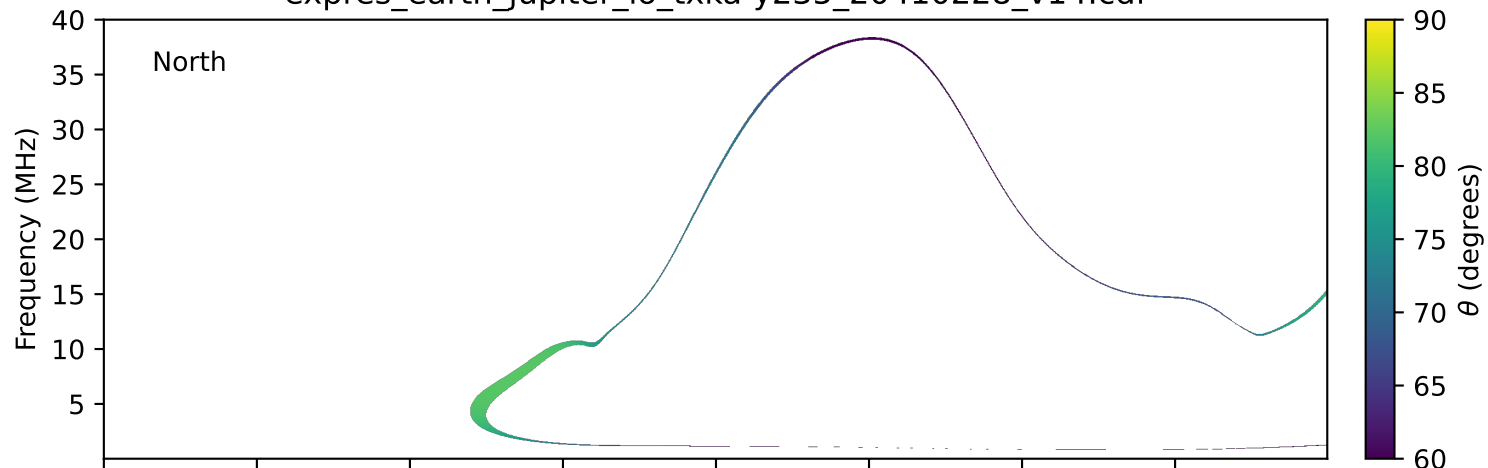
expres_earth_jupiter_io_txka-y235_20410228_v14.cdf
