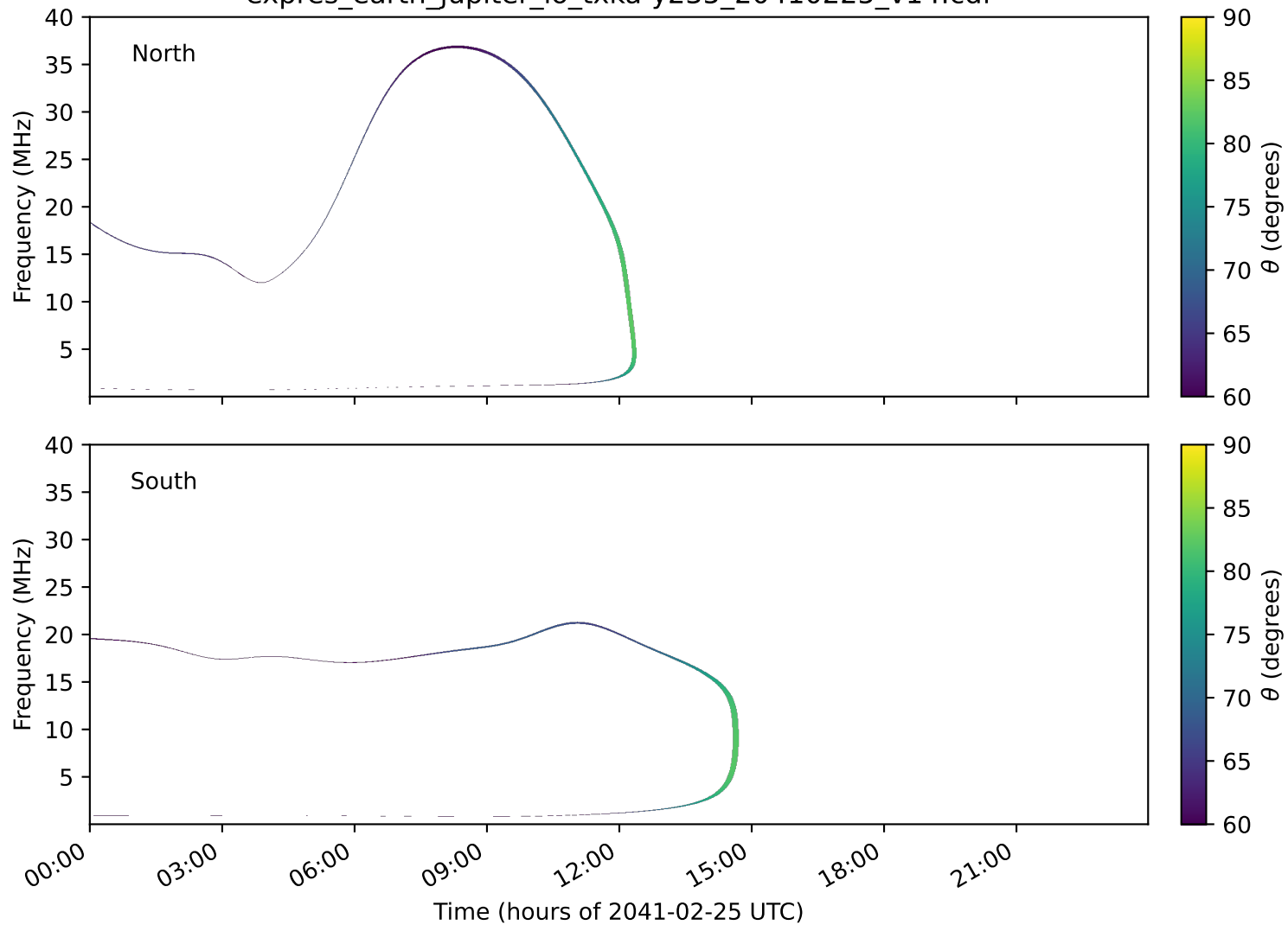
expres_earth_jupiter_io_txka-y235_20410225_v14.cdf
