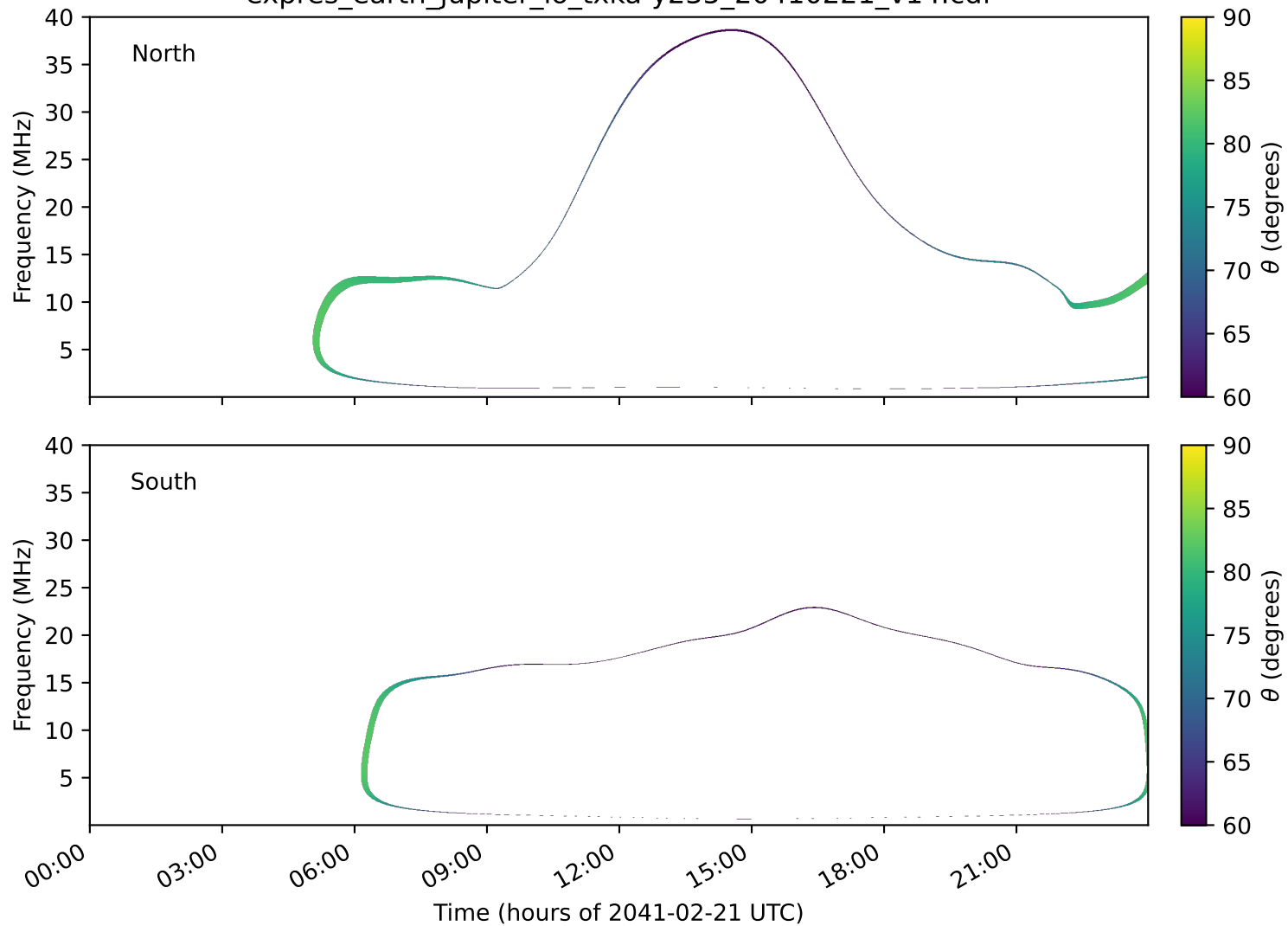
expres_earth_jupiter_io_txka-y235_20410221_v14.cdf
