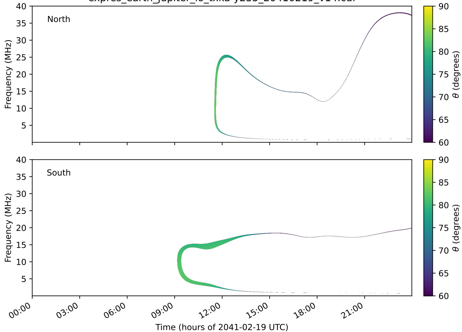
expres_earth_jupiter_io_txka-y235_20410219_v14.cdf
