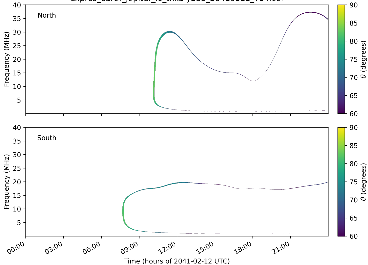
expres_earth_jupiter_io_txka-y235_20410212_v14.cdf
