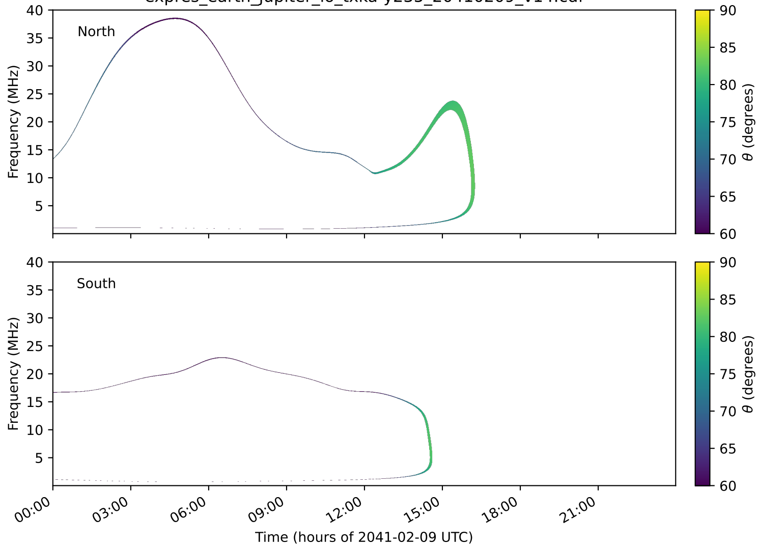
expres_earth_jupiter_io_txka-y235_20410209_v14.cdf
