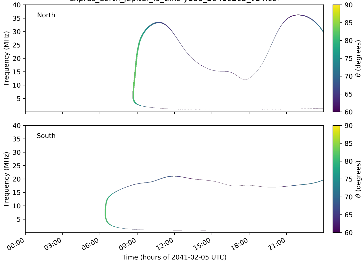
expres_earth_jupiter_io_txka-y235_20410205_v14.cdf
