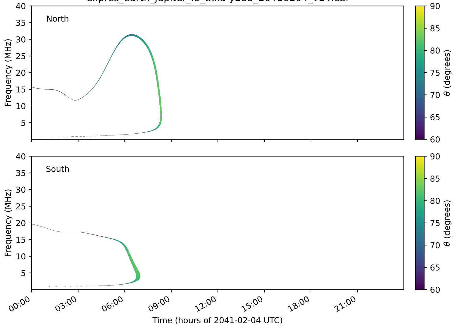
expres_earth_jupiter_io_txka-y235_20410204_v14.cdf
