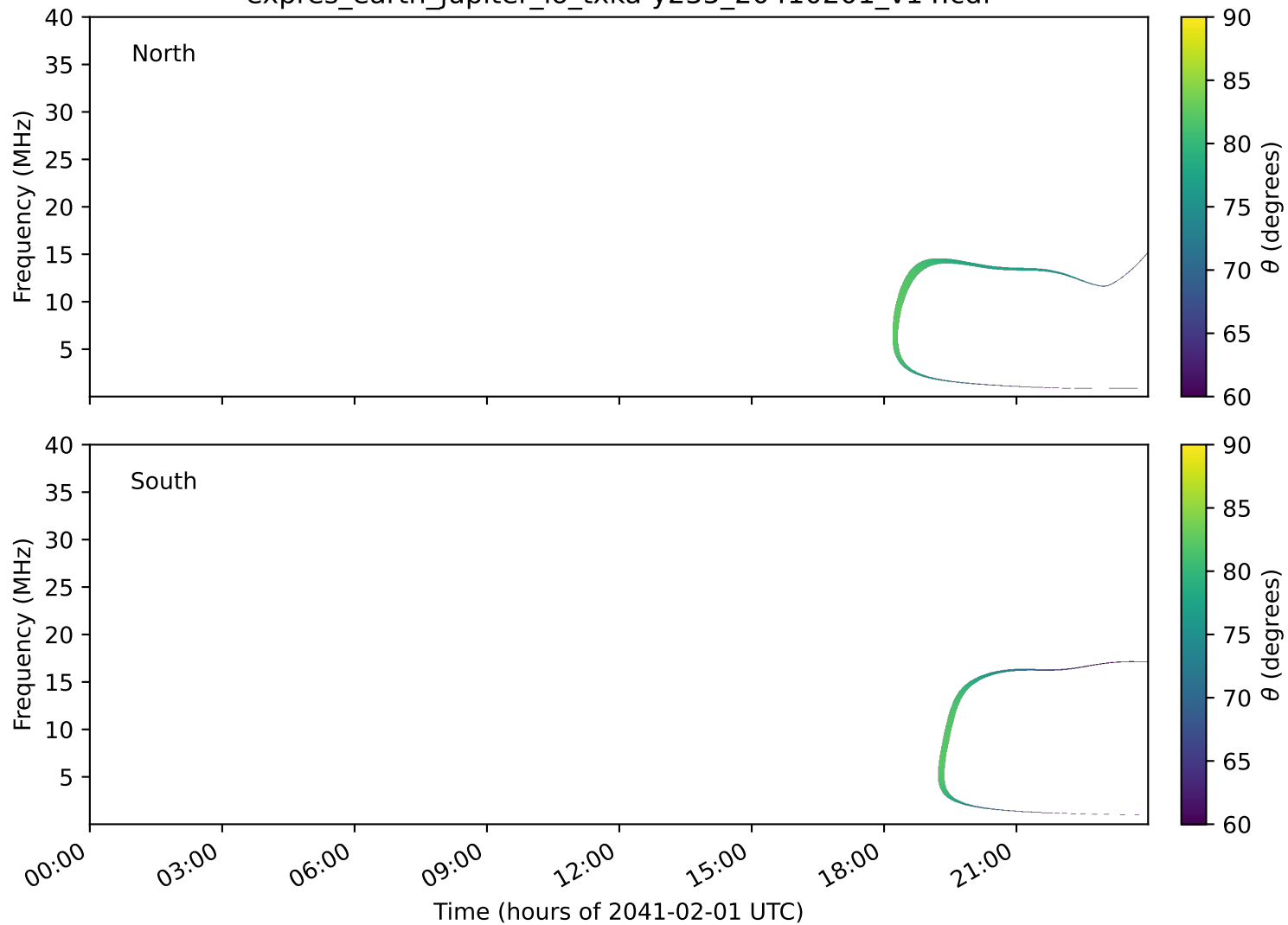
expres_earth_jupiter_io_txka-y235_20410201_v14.cdf
