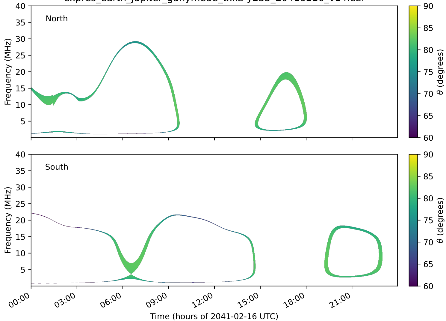
expres_earth_jupiter_ganymede_txka-y235_20410216_v14.cdf
