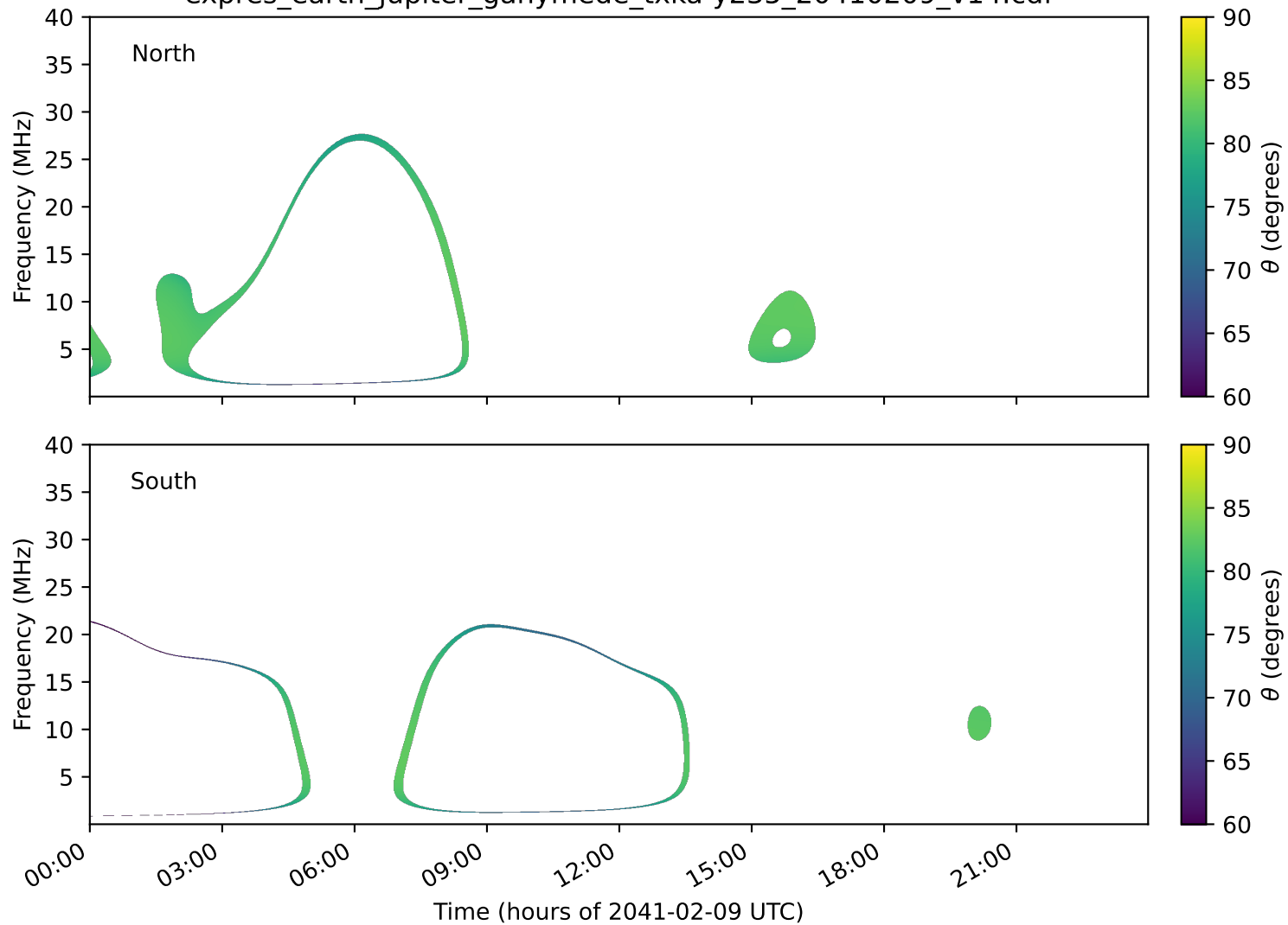
expres_earth_jupiter_ganymede_txka-y235_20410209_v14.cdf
