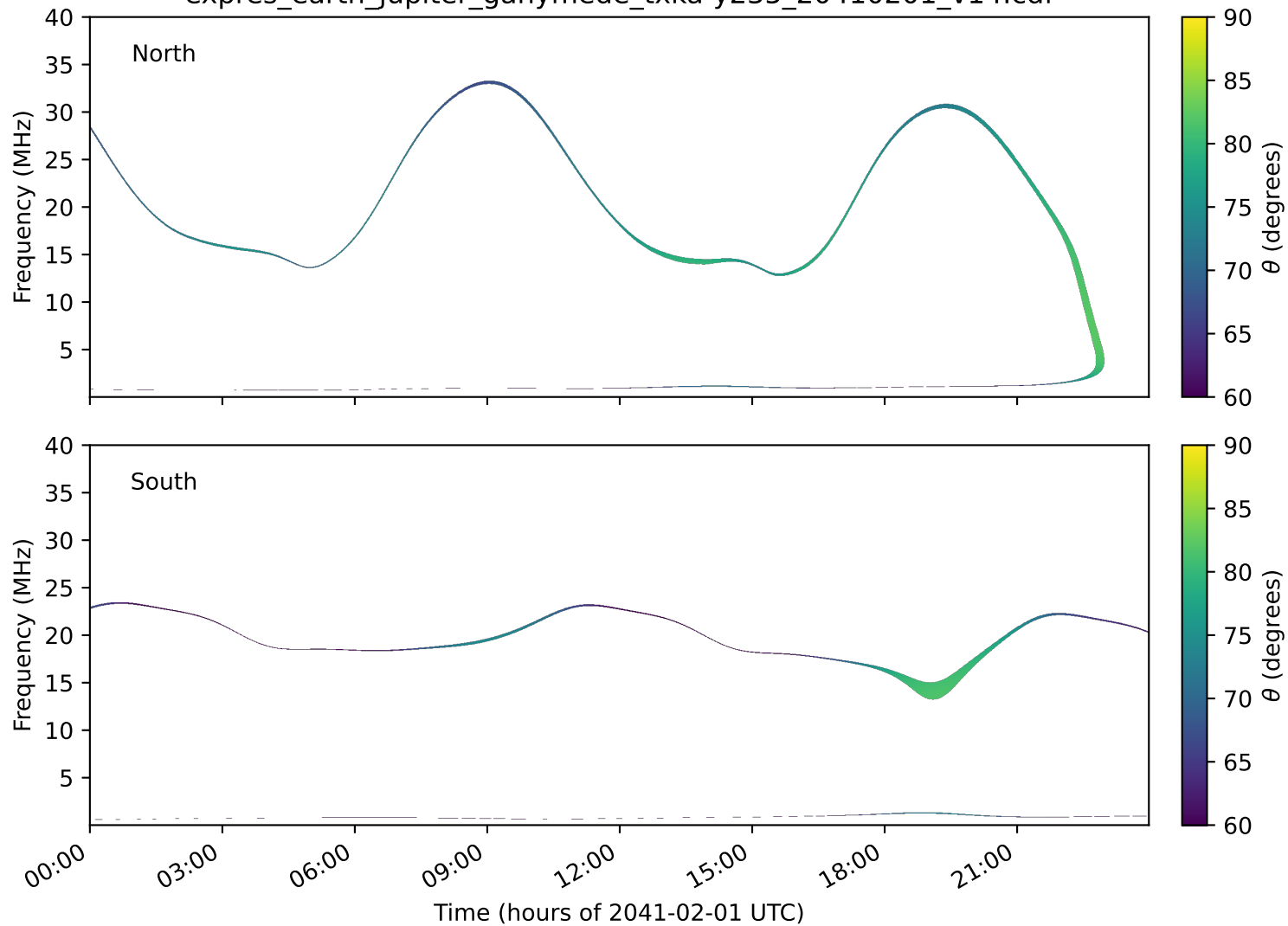
expres_earth_jupiter_ganymede_txka-y235_20410201_v14.cdf
