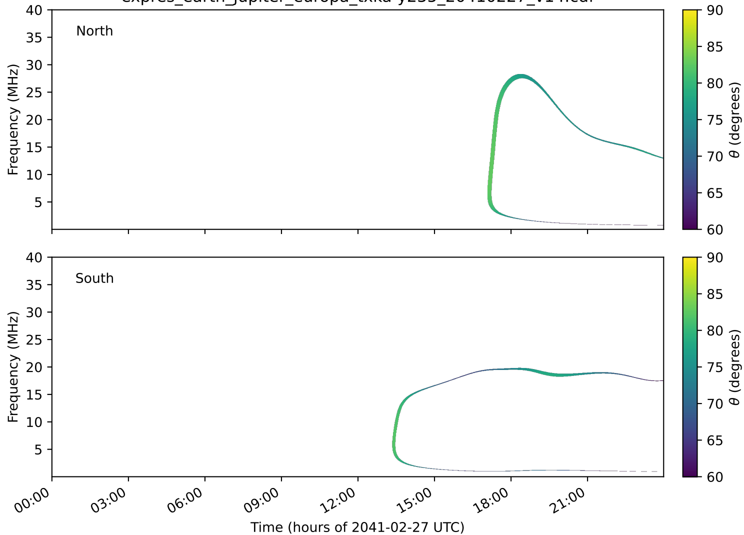
expres_earth_jupiter_europa_txka-y235_20410227_v14.cdf
