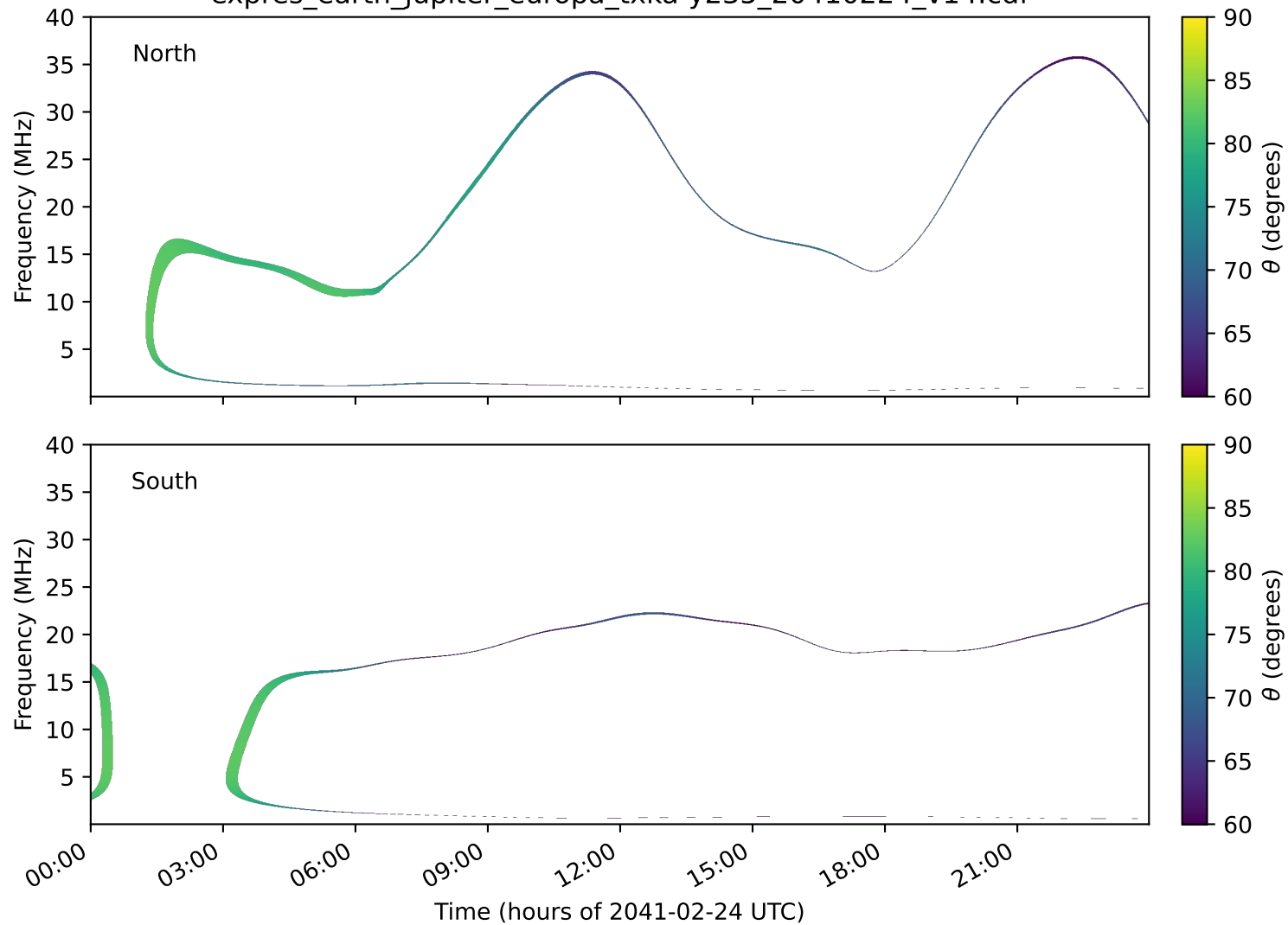
expres_earth_jupiter_europa_txka-y235_20410224_v14.cdf
