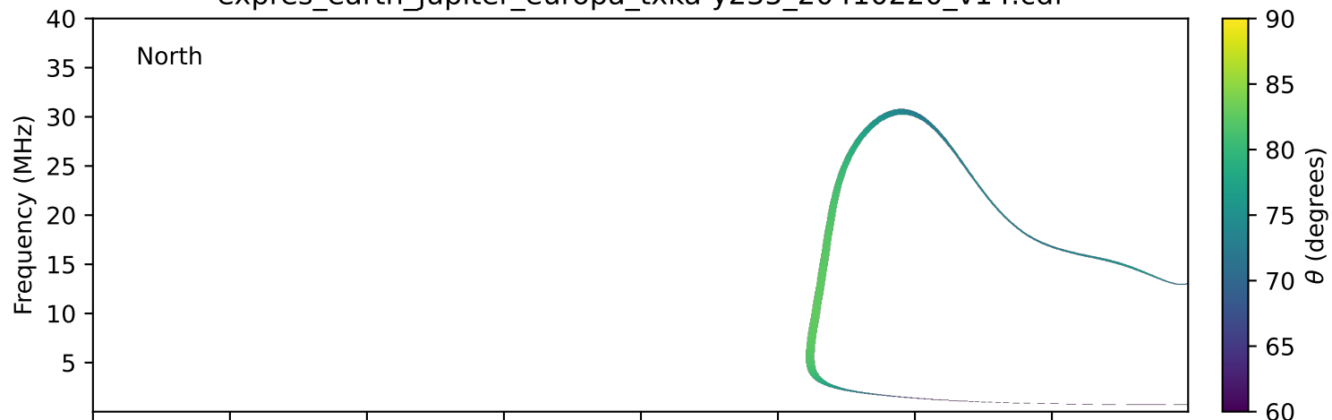
expres_earth_jupiter_europa_txka-y235_20410220_v14.cdf
