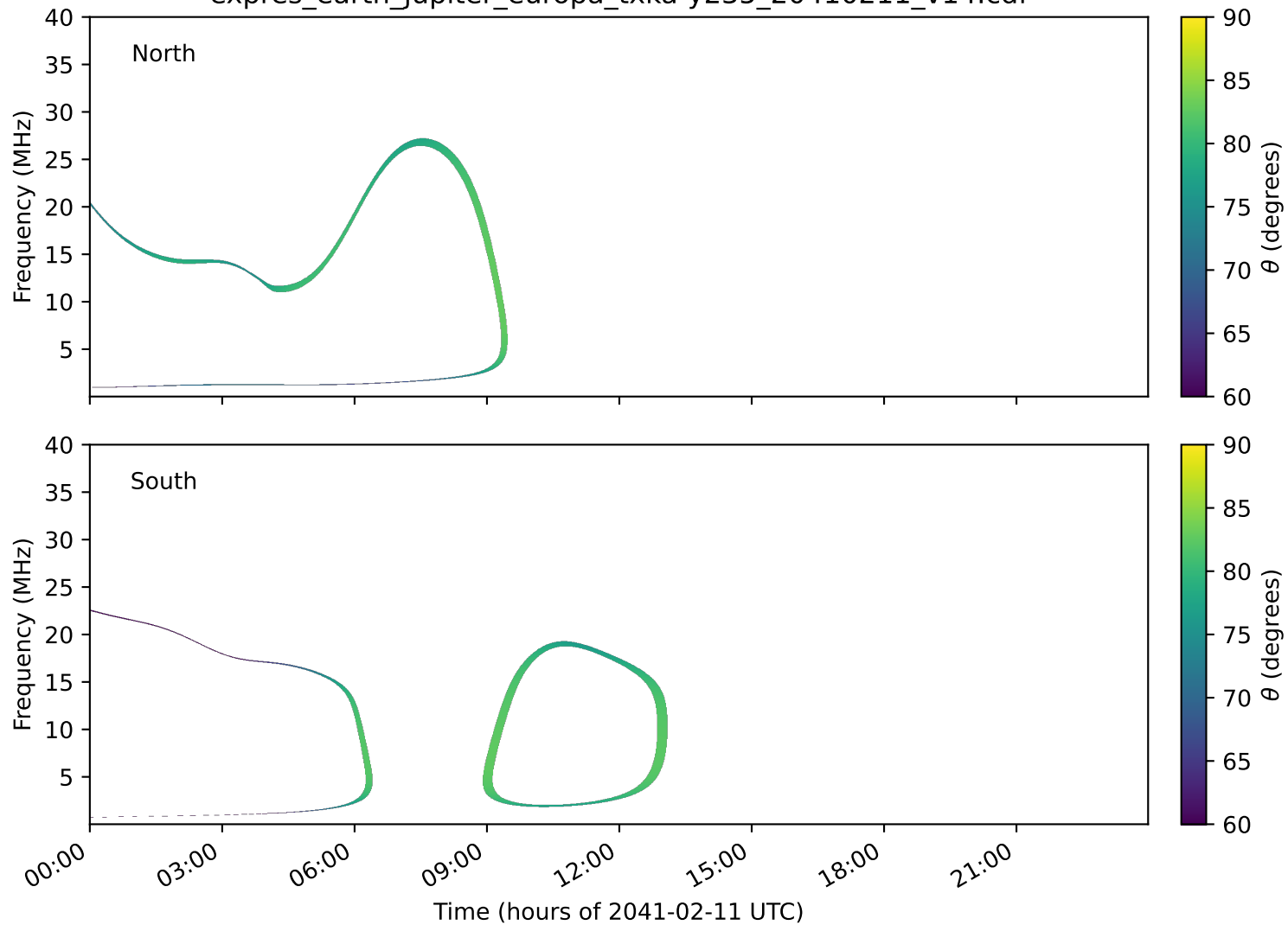
expres_earth_jupiter_europa_txka-y235_20410211_v14.cdf
