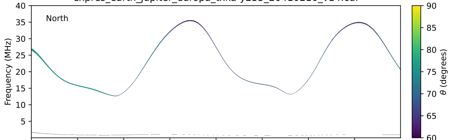
expres_earth_jupiter_europa_txka-y235_20410210_v14.cdf
